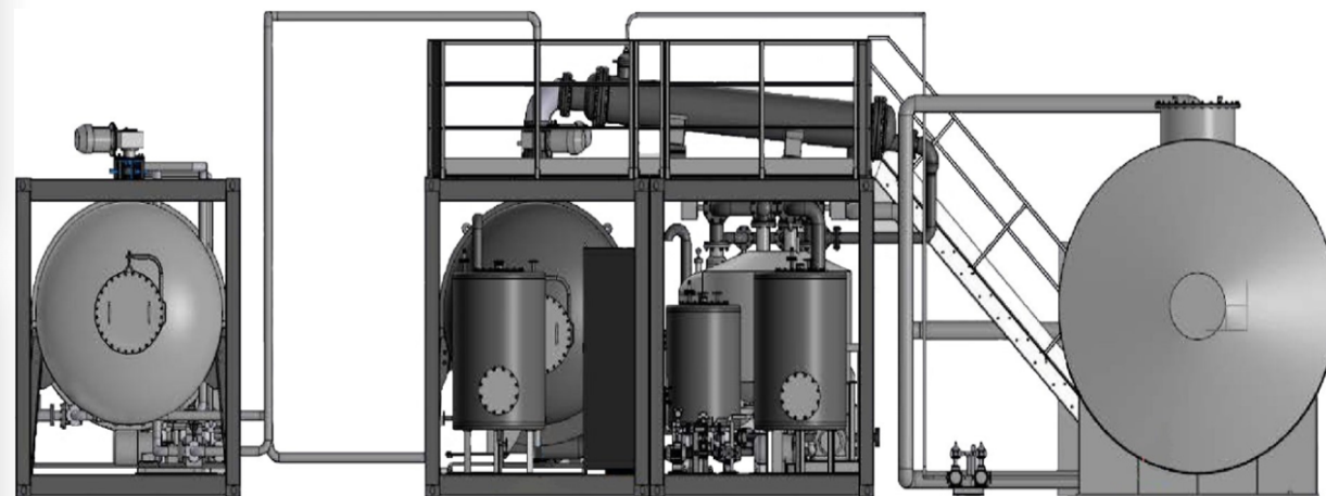
Mobile plant for processing. Capacity – 3000 tons per year
